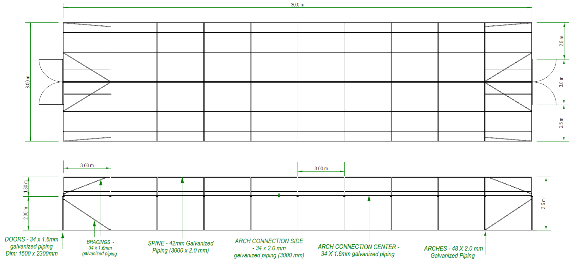
SIDE ELEVATION
