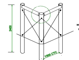
CORNER BOX
