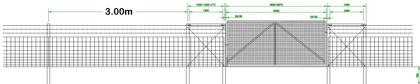
B FENCE LINE WITH SINGLE VEHICLE GATE
