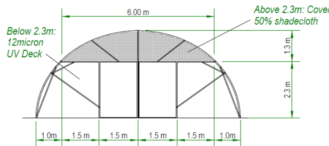
FRONT/BACK ELEVATION
