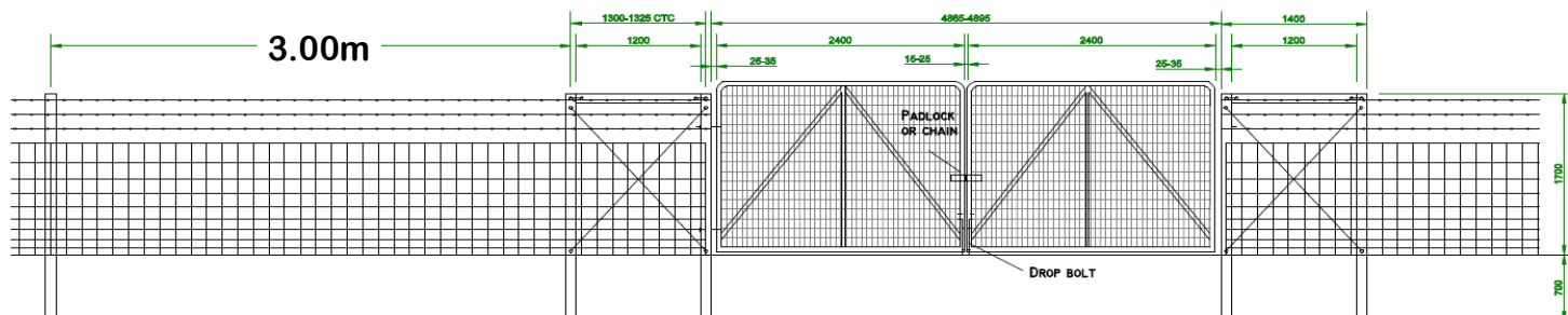
C FENCE LINE WITH DOUBLE TRACTOR GATE
